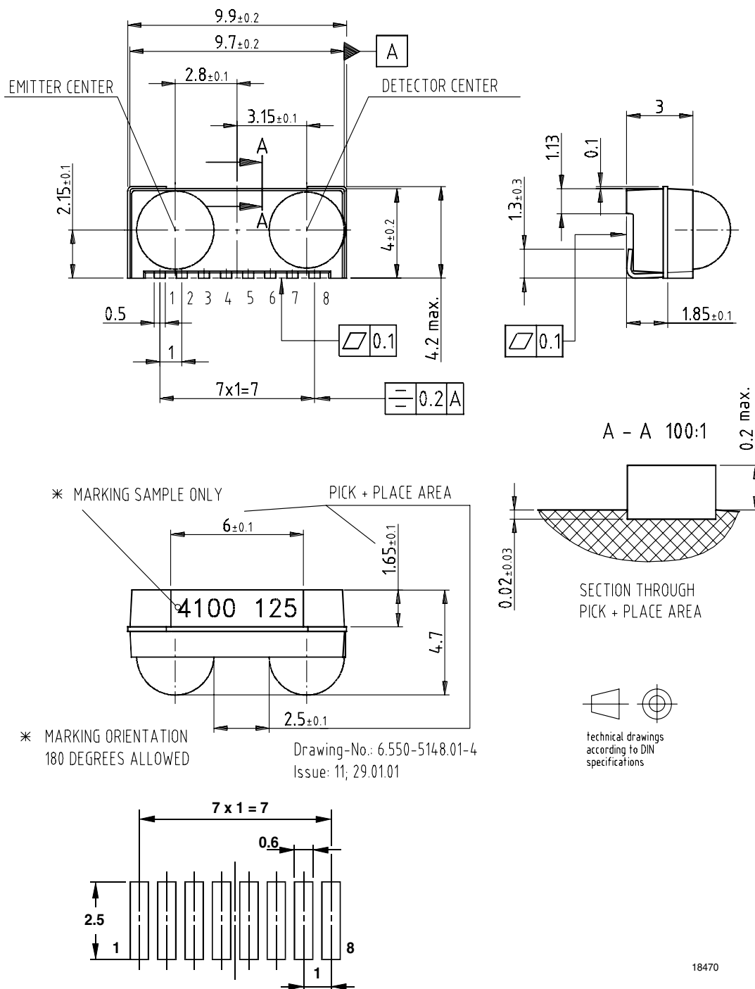
Figure 7. Package drawing TFDU6103, dimensions in mm, tolerance \pm 0.2 mm if not otherwise mentioned
